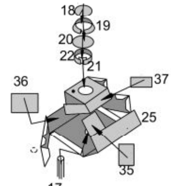
TSF Superstructure
